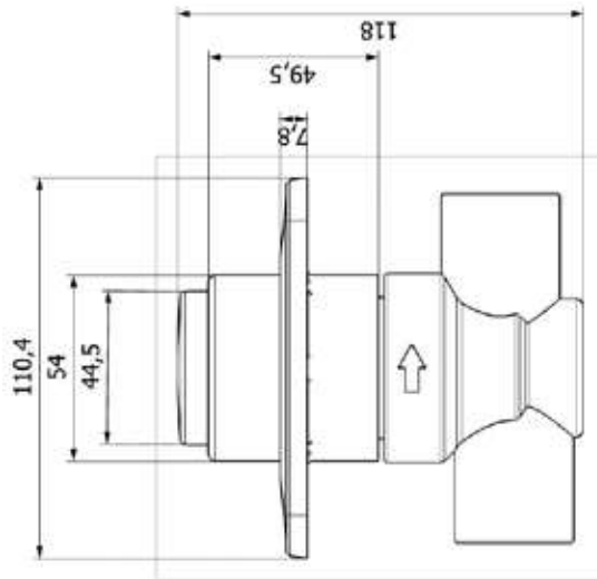
TK 020 - 25 mm (3/4) / TK 021 - 32 mm (1")
